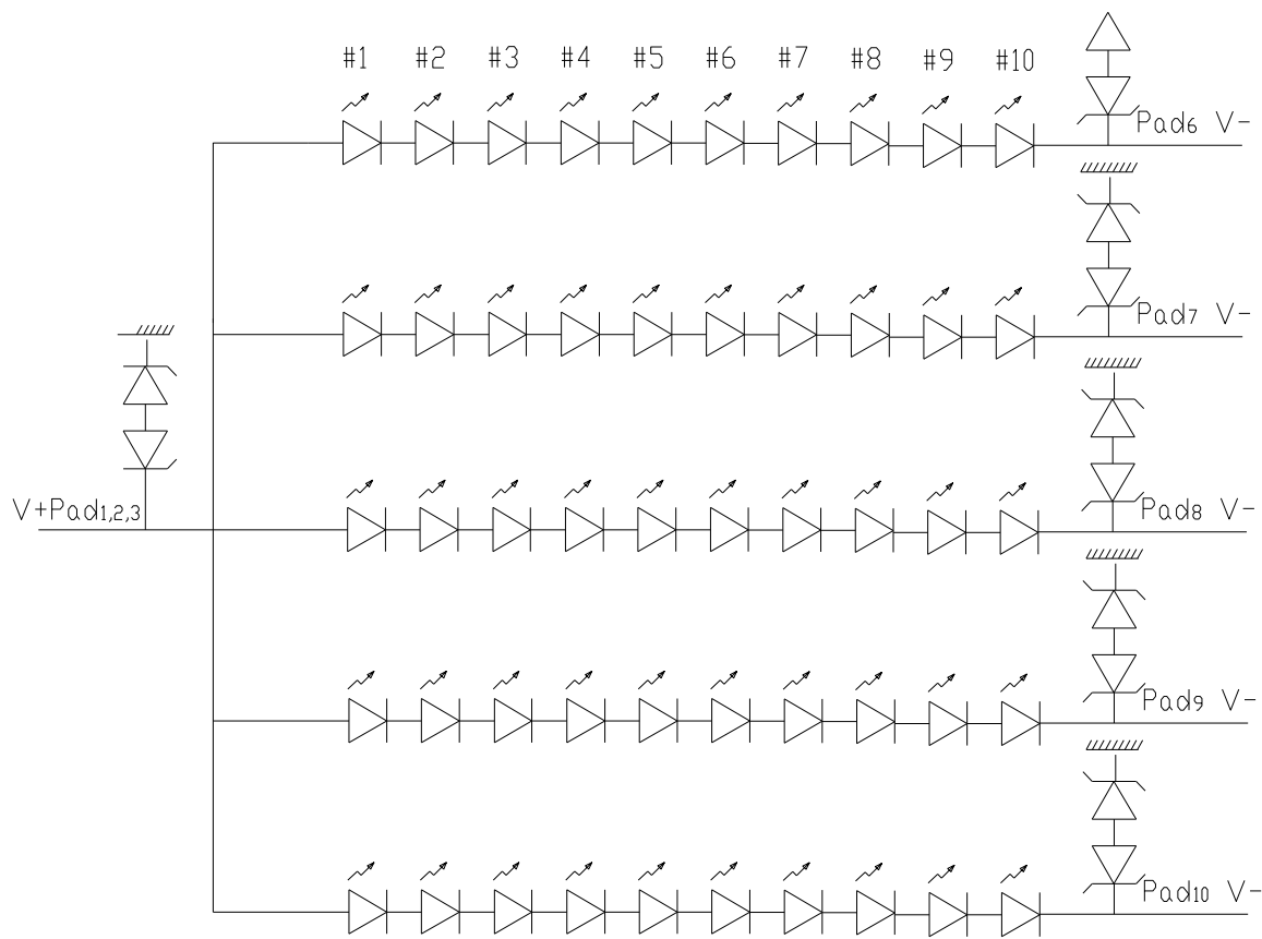
Figure 6. LED Structure
