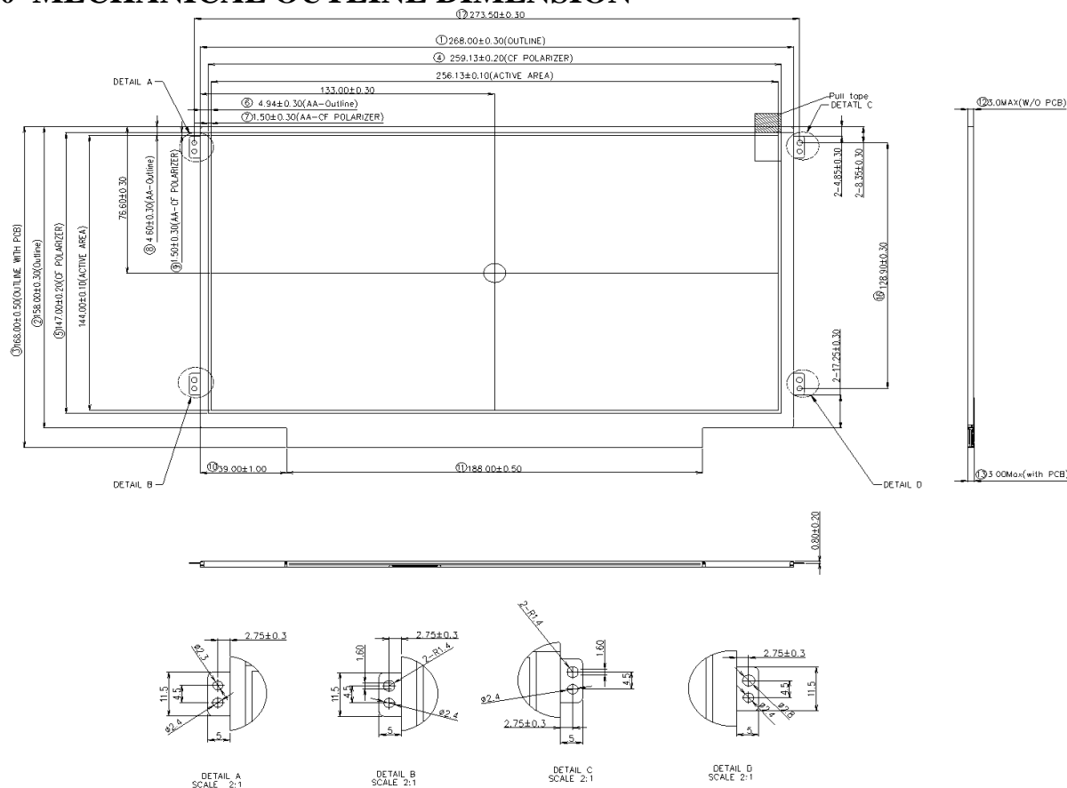
Figure 23. TFT-LCD Module Outline Dimension (Front View)
